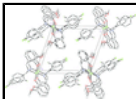
Fig. 2. A crystal packing diagram of the title compound, viewed along the a axis.
